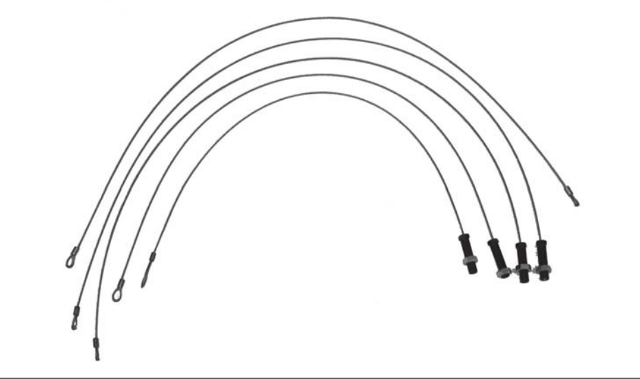
Moving deck cable assembly Product Code B12100280000 EA Upper scissors cable Product Code B12200066002 EA Upper deck cable Product Code B12200066003 EA Lower deck cable Product Code B12200066004 EA Lower Scissors Cable Product Code B12200067000 EA
